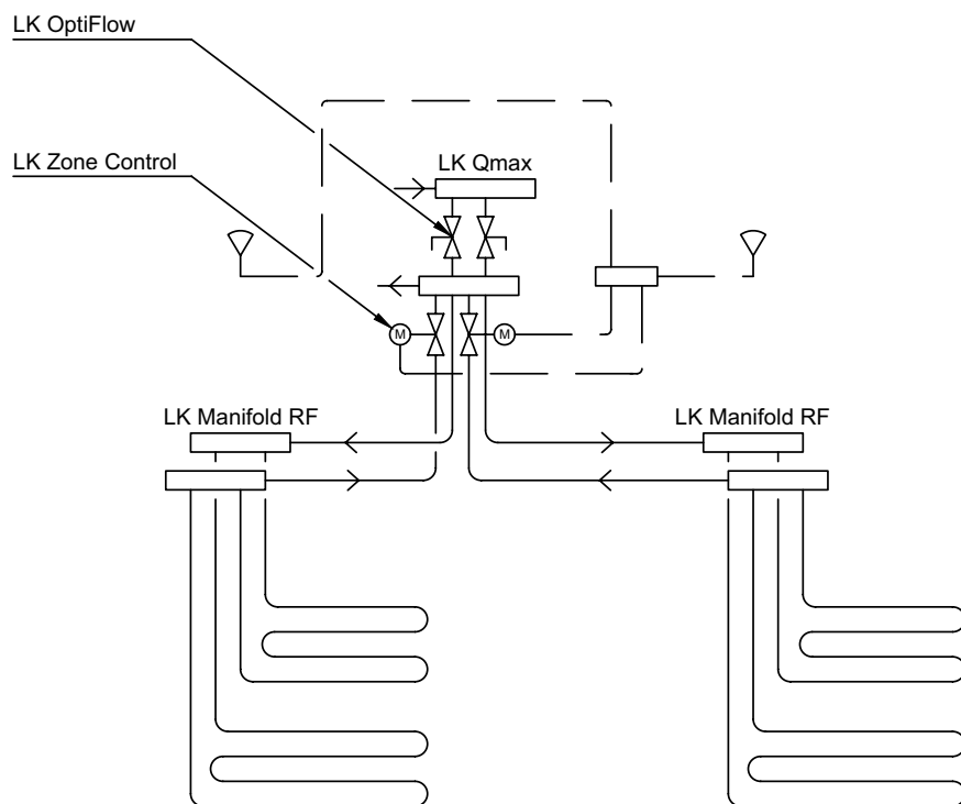
LK Zone Control against LK Qmax.
