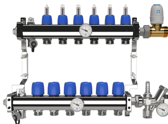
LK Zone Control straight design right.
