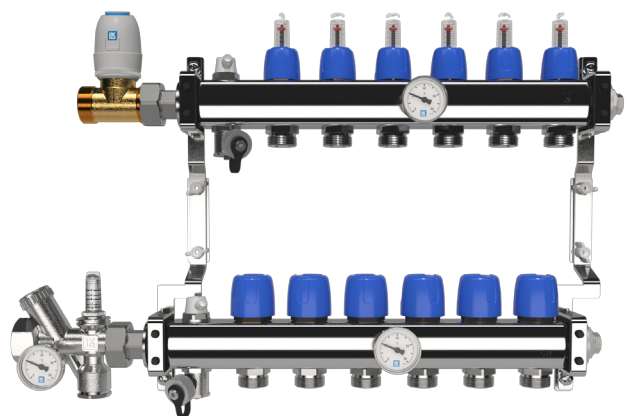
LK Zone Control straight design left.
