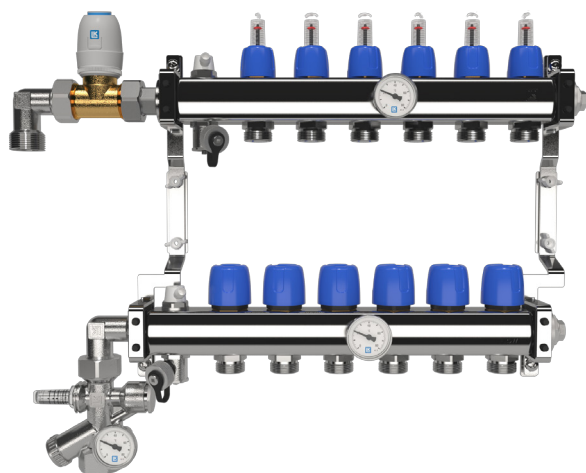
LK Zone Control angled design left.
